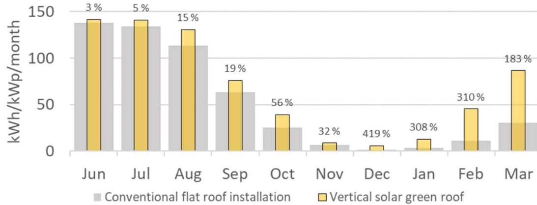
Energy yield per month (% gain)
